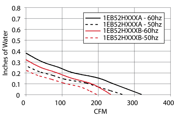
1EB Models
