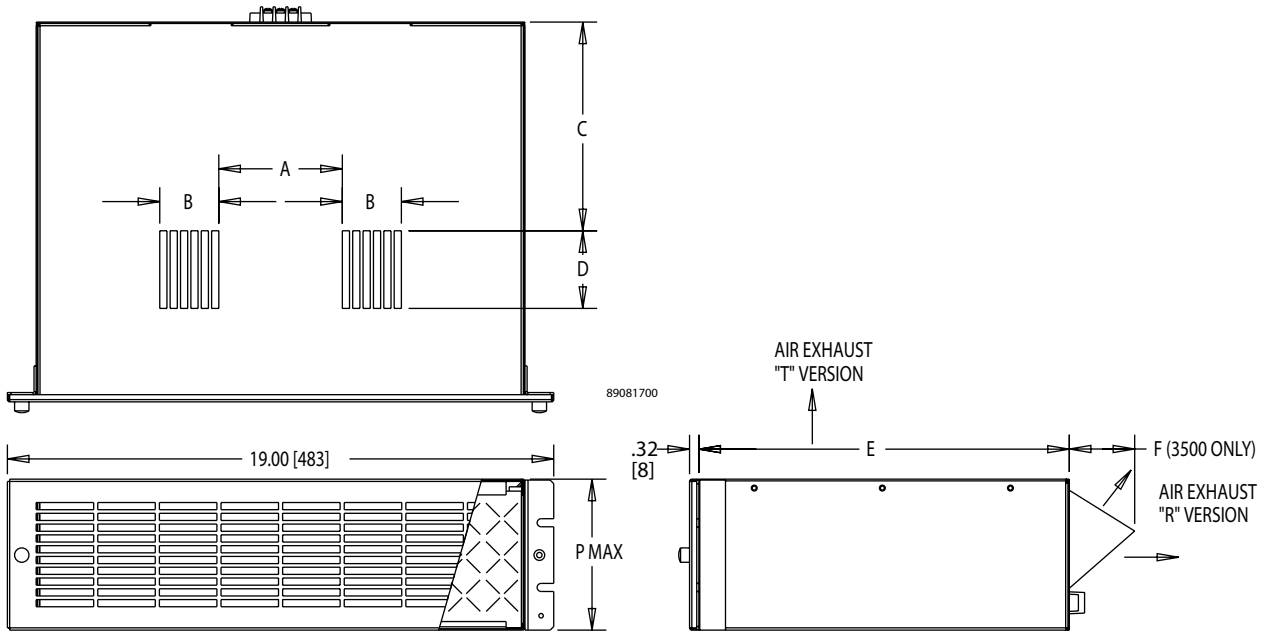
4EB Models
