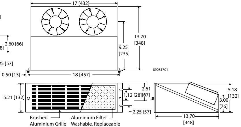
1EB52HxxxA Models
