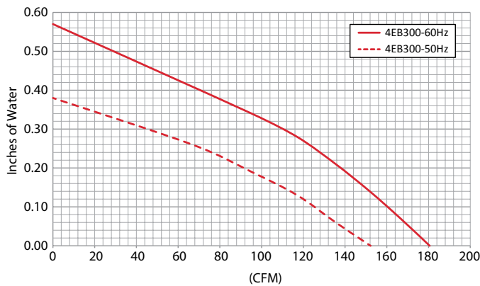
4EB Models
