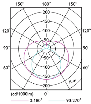
Light Distribution Diagram - 15T8/COR/48-850/MF21/G/120-347V 25/1
