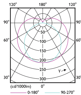
Light Distribution Diagram - 14T8/48-840/IF21/MC IA 10/1
