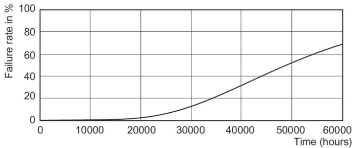
Life Expectancy Diagram - 35T8/96-4000 IF FA8 10/1
