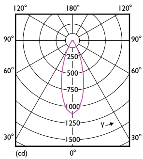
Light Distribution Diagram - 5.5PAR20/LED/F40/927-922/DIM/G/T20 6/1FB
