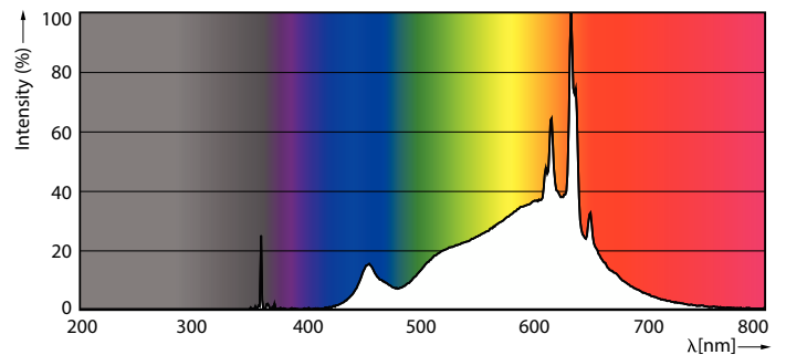
Spectral Power Distribution Colour - 5.5PAR20/LED/F40/927-922/DIM/G/T20 6/1FB
