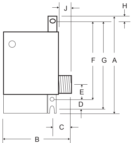
DEVANT | FRONT
