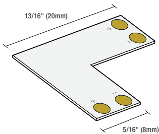
67630 - L SHAPE PCB JOINER
