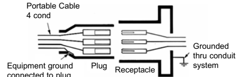
Style 1: 3-wire, 3-pole
