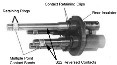
Figure 10. Suffix S22 Reversed Contacts
