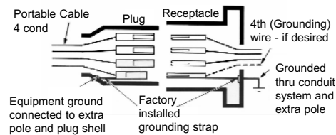
Style 2: 3-wire, 4-pole
