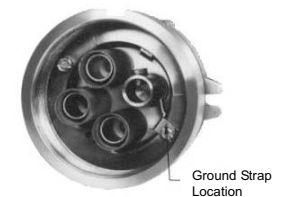
Figure 9. Grounding Strap Location
