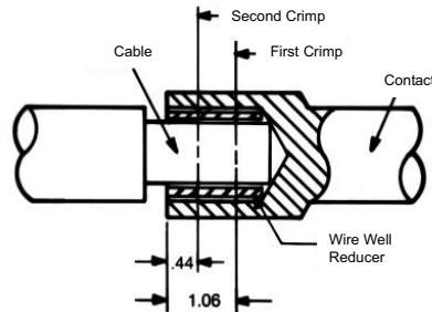
Figure 7. Crimp Connection
