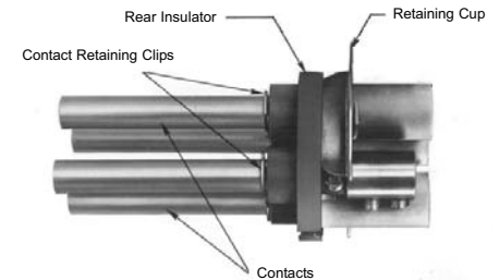
Figure 8. Retaining Clip Locations
