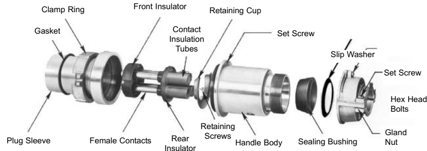
Figure 1. AP Plug Detailed Description (Style 2 Shown)
