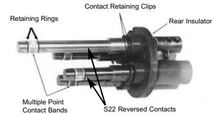
Figure 10. Contacts inversés (suffixe S22)
