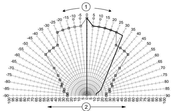
Figure 4: UL 1971 minimum light output (% of rating vs. angle)
