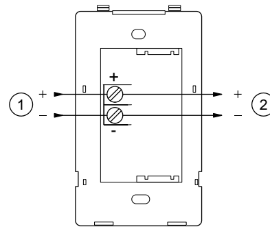
Figure 3: Wiring diagram
