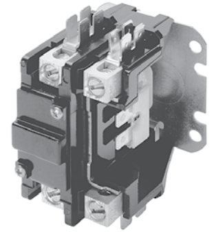
Series CDP2 1-pole contactor
