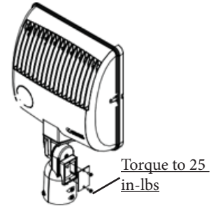
DSXF3 (Integral slipfitter)
