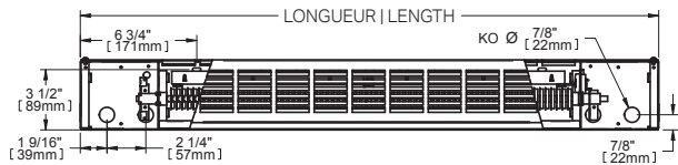
DEVANT | FRONT
