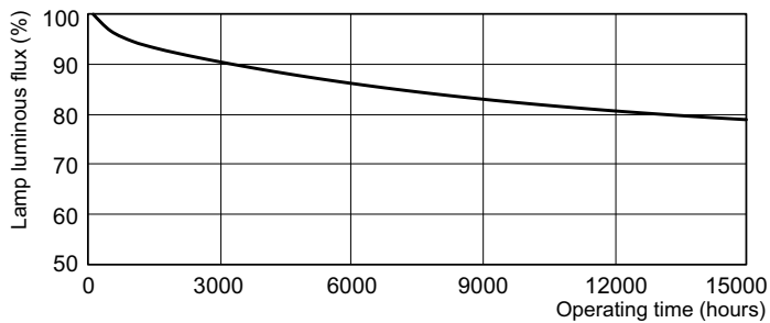
Lumen Maintenance Diagram - PL-T 42W/827/A/4P 1CT/5X10BOX ALTO
