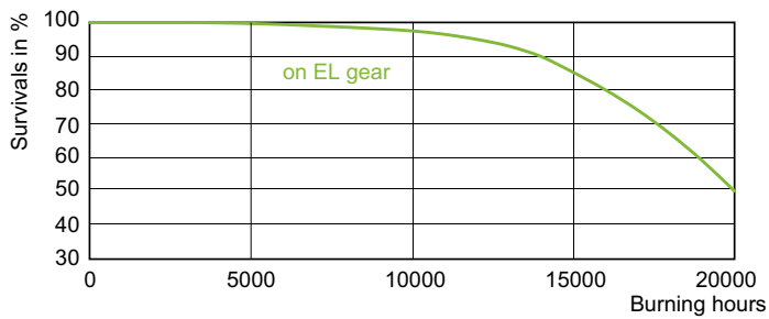
Life Expectancy Diagram - MASTERColor CDM-T Elite 70W/930 G12 1CT
