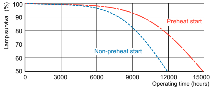
Life Expectancy Diagram - PL-C 13W/830/4P/ALTO 10PK
