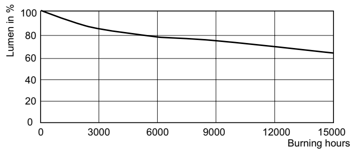
Lumen Maintenance Diagram - CDM-TD 70W/830 RX7s T6 CL
