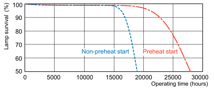
Life Expectancy Diagram - 39W/835 Min Bipin T5 HO ALTO UNP
