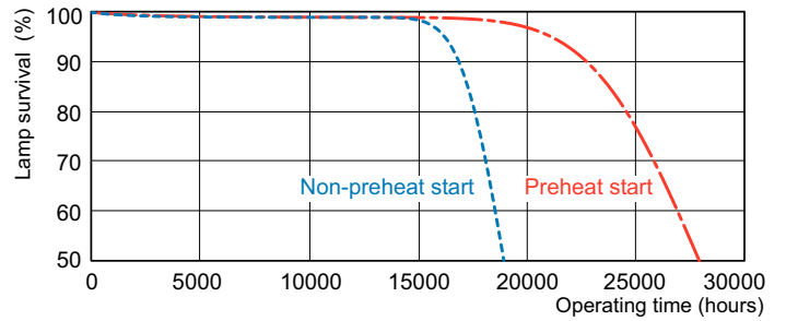
Life Expectancy Diagram - 39W/830 Min Bipin T5 HO ALTO UNP
