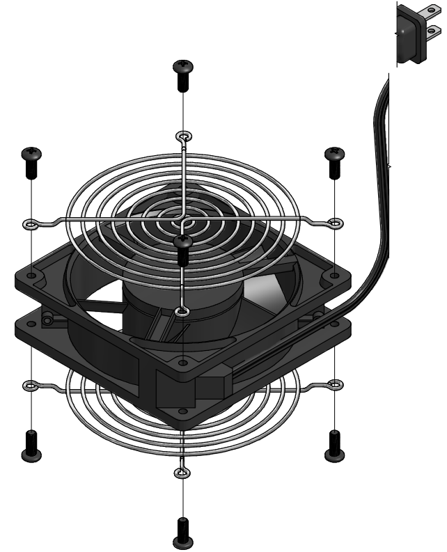
EXPLODED ASSEMBLY VIEW
