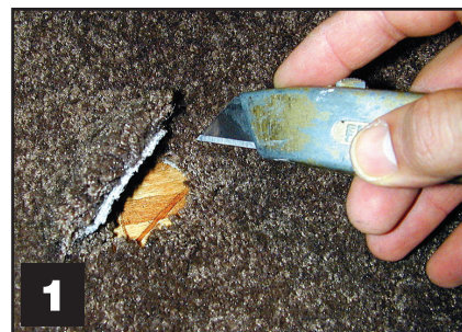
Figure 1 - Cut 2-3/8" hole through carpeting before using a hole saw.
