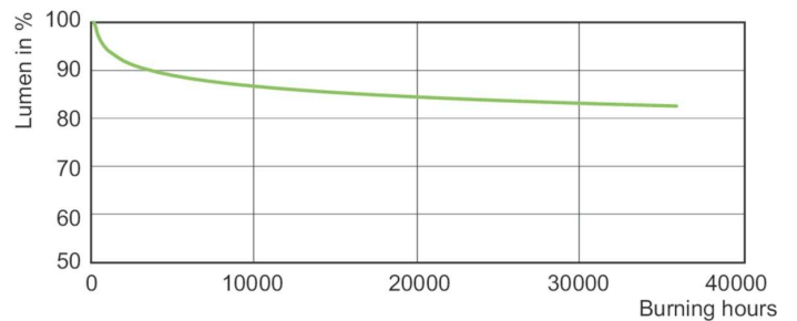
Lumen Maintenance Diagram - Allstart Energy Adv 330W ED37 CL 1SL
