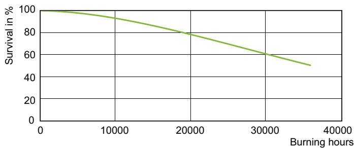
Life Expectancy Diagram - Allstart Energy Adv 330W ED37 CL 1SL
