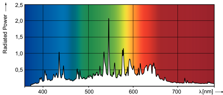
Spectral Power Distribution Colour - Allstart Energy Adv 330W ED37 CL 1SL
