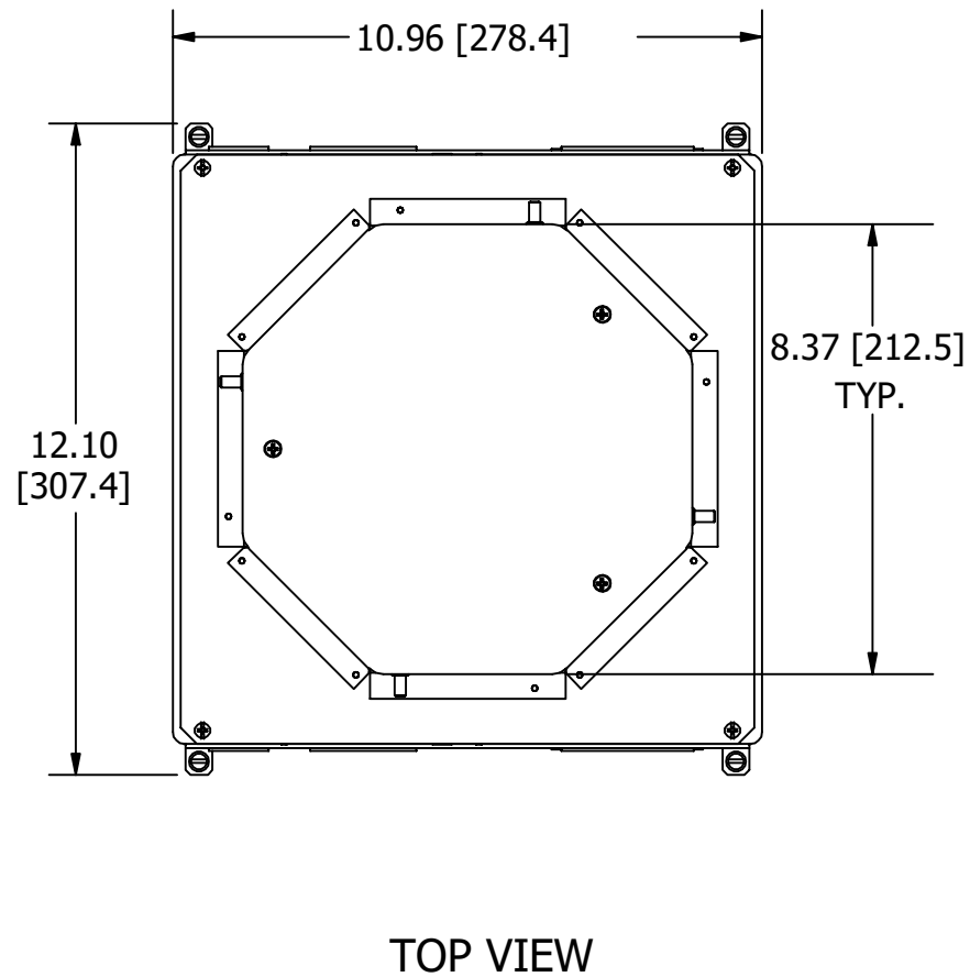
CFB10G55R / CFB10G55RCR (ROUND COVER FOR 6.25" MIN POUR)
