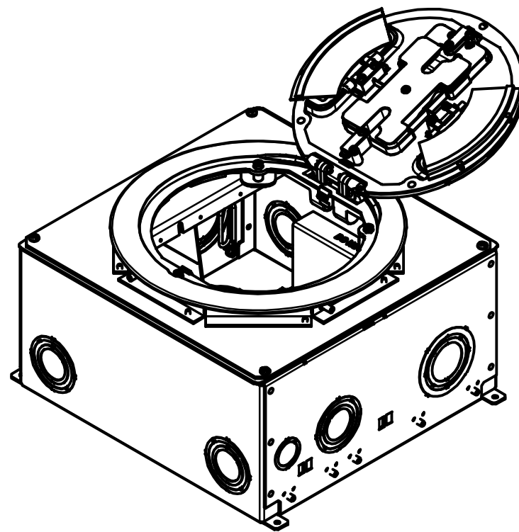
CFB10G55R / CFB10G55RCR (ROUND COVER OPEN)
