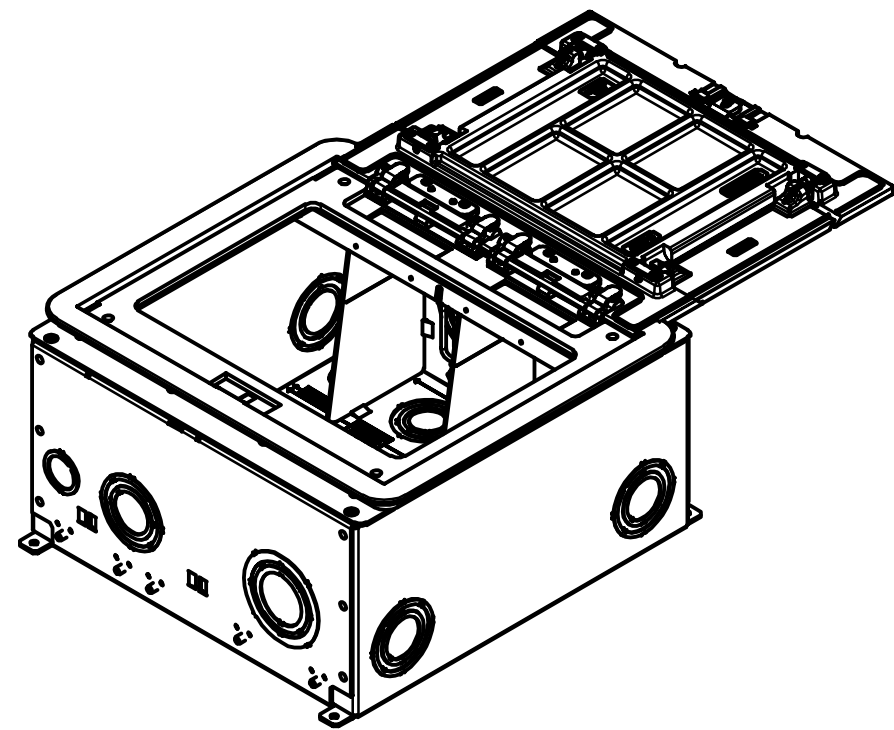
CFB10G55 / CFB10G55CR (RECTANGULAR COVER OPEN)
