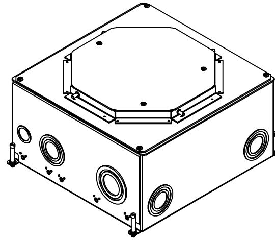
CFB10G55R / CFB10G55RCR (ROUND COVER FOR 6.25" MIN POUR)
