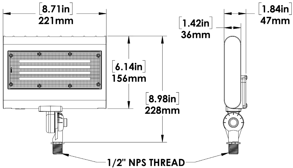
Knuckle Mount
