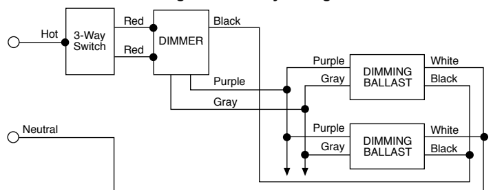
Figure 2 – 3-Way Wiring
