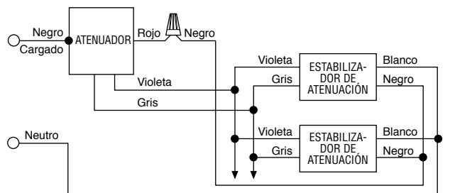
Figura 1 – Cableado unipolar
