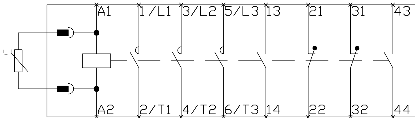
LENOOF G & H Wiring Diagram
