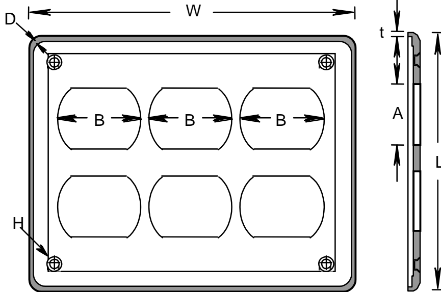
TRIPPLE RECEPTACLE, TYPE DRC20-3 CODE: 077747
