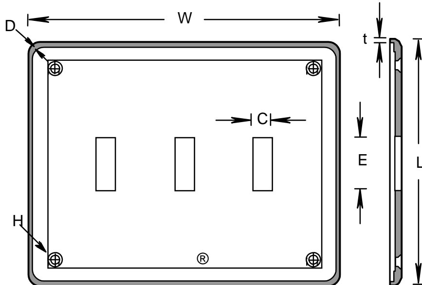
TRIPPLE SWITCH, TYPE TSC20-3 CODE: 077744
