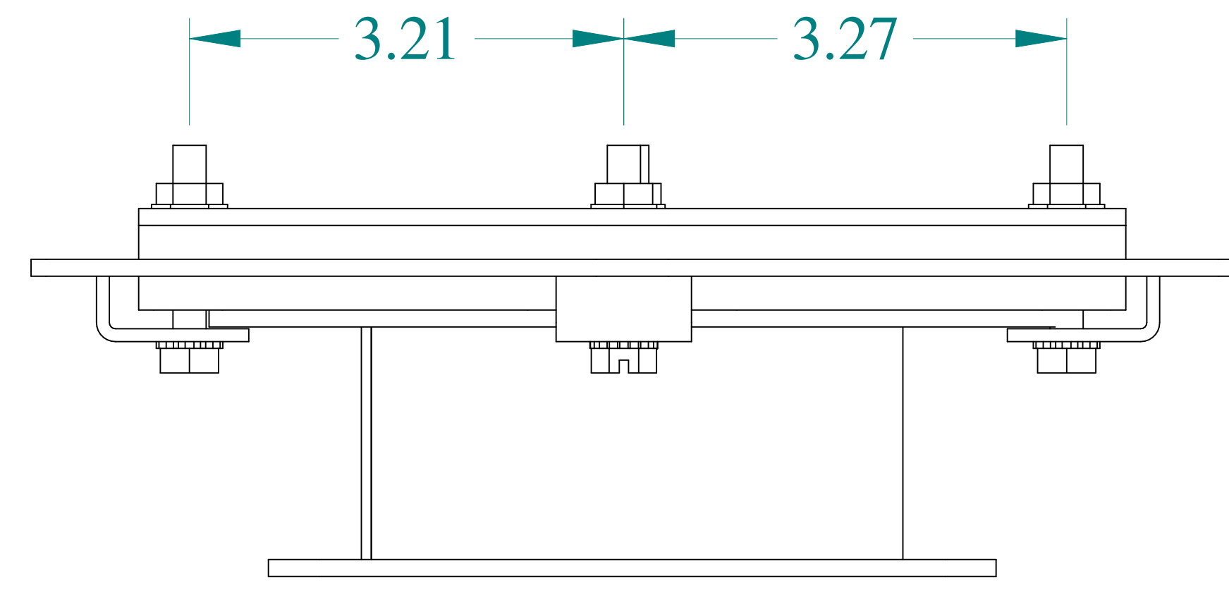
TOP VIEW
