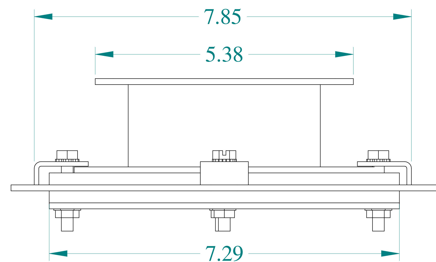
BOTTOM VIEW
