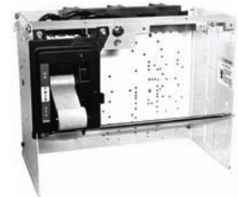
F2100 Feeder Unit
