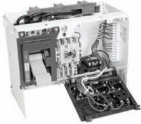
Unit with Freedom Starter
