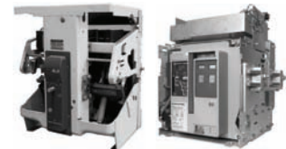
Original AK-2A-50 AK2A50-AR1600M
