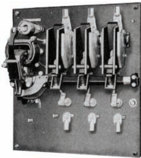
Size 5 Contactor
