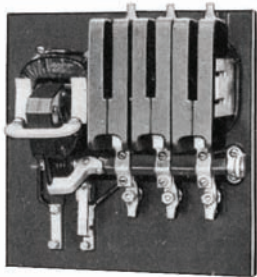
Size 2 Contactor
