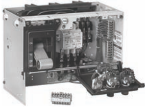
Unit with A200 Starter
