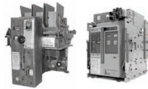
Original LA-600 LA600-AR600NM
