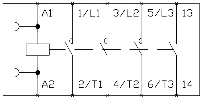
LEN00B003 Wiring Diagram
