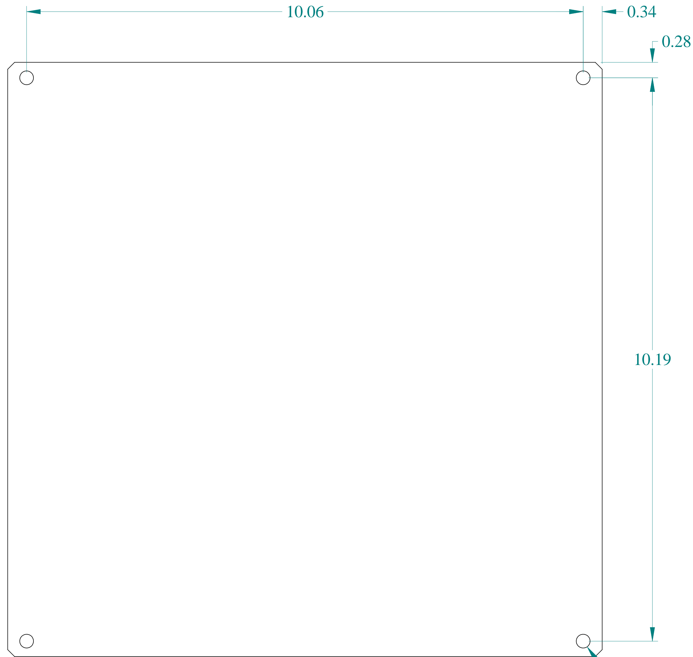
FRONT VIEW
