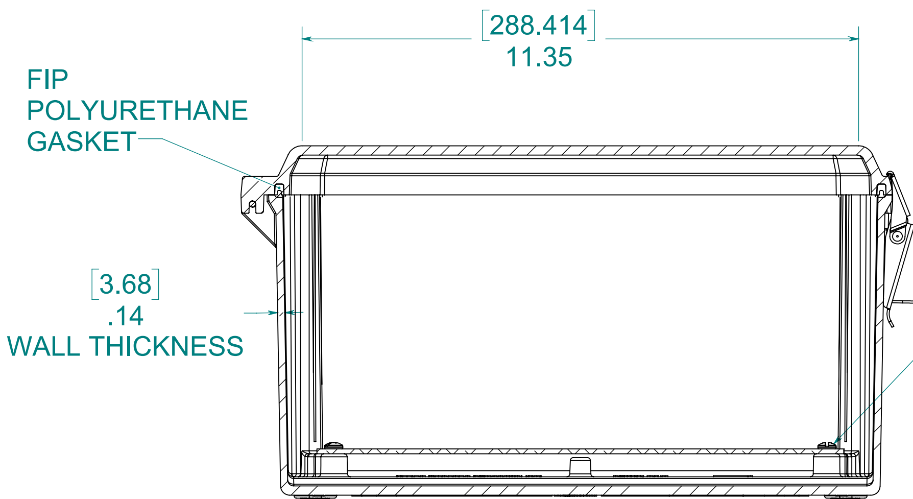
SECTION B-B
