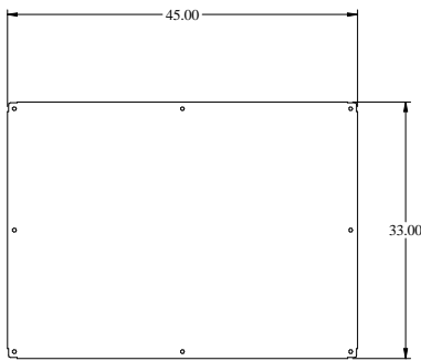
INNER PANEL
