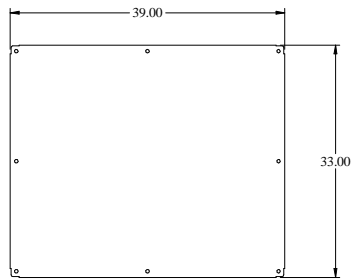
INNER PANEL
