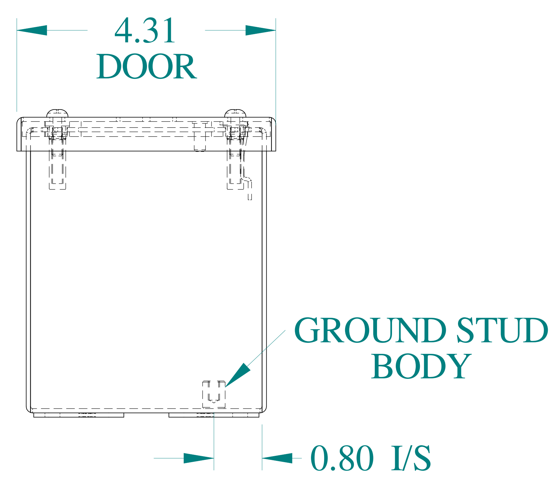
BOTTOM VIEW
