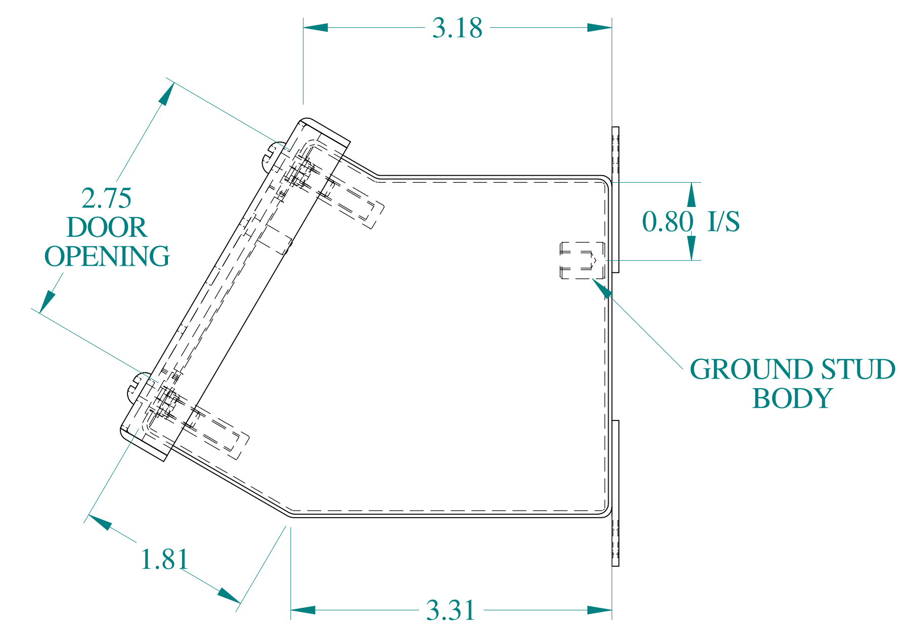
SIDE VIEW
