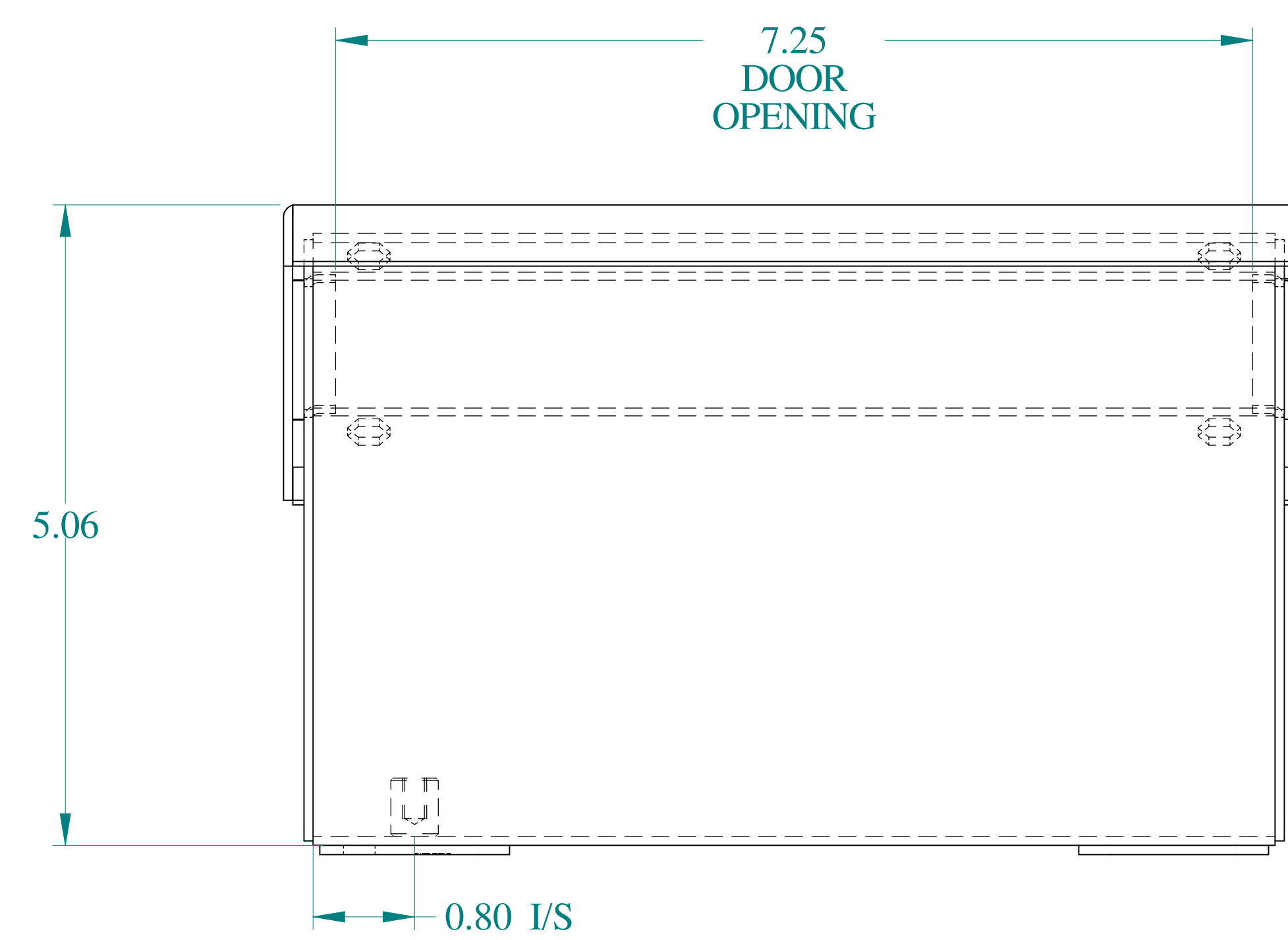
BOTTOM VIEW
