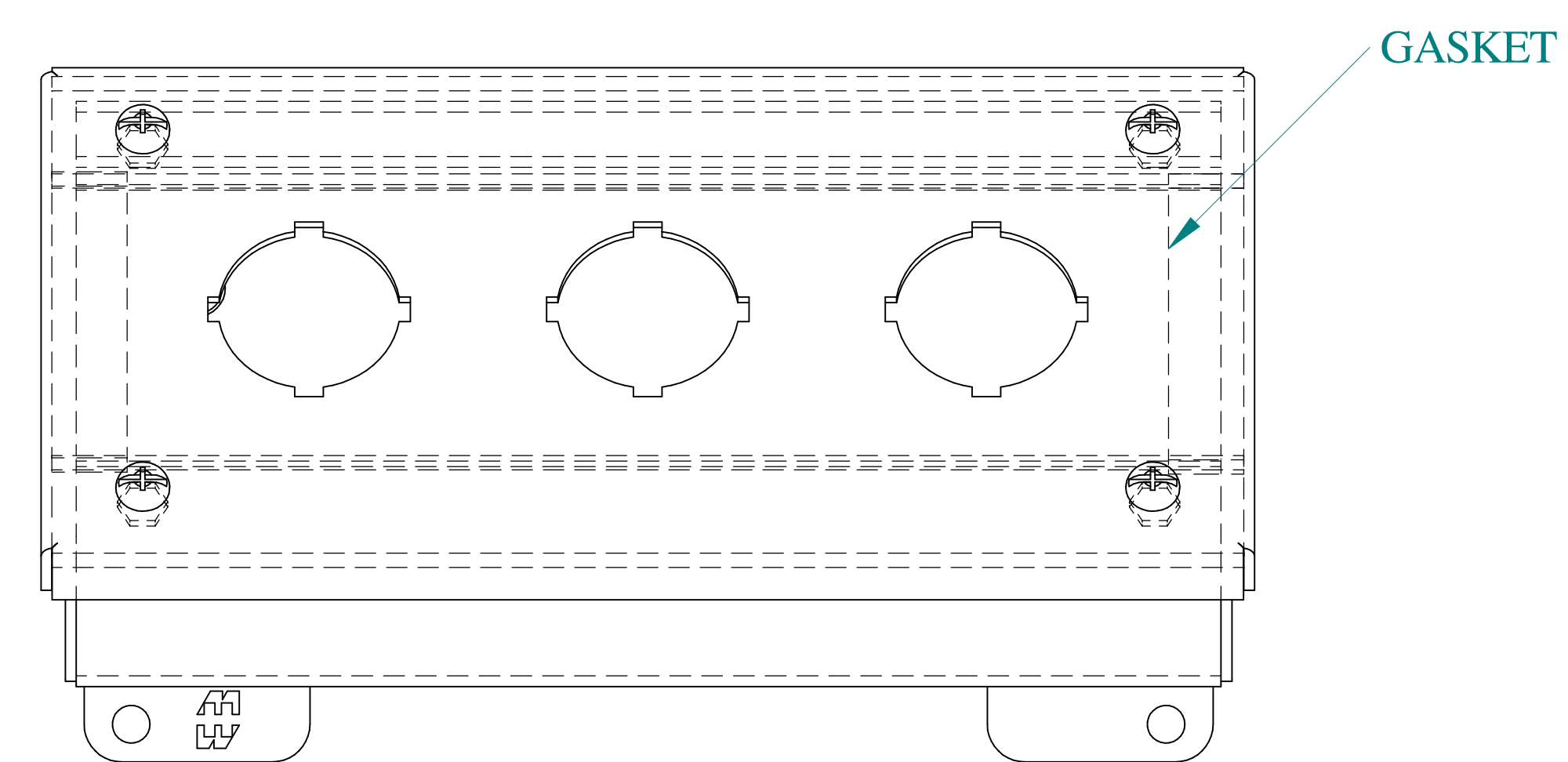
FRONT VIEW
