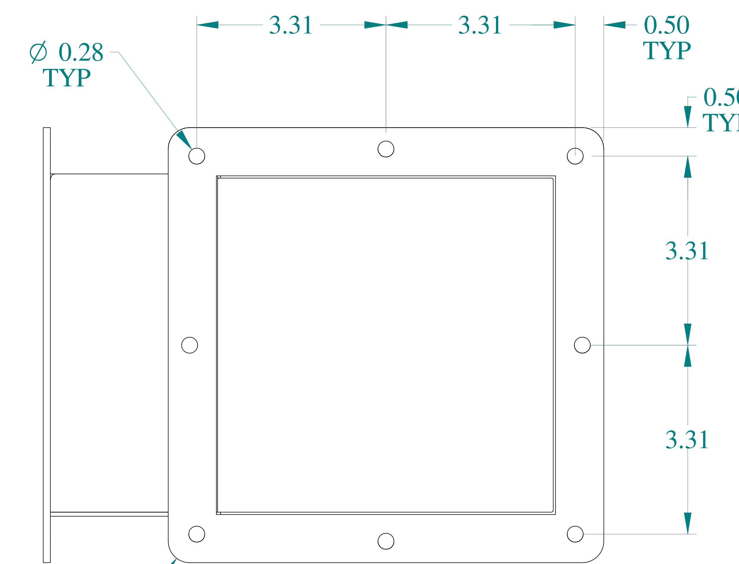
SIDE VIEW
