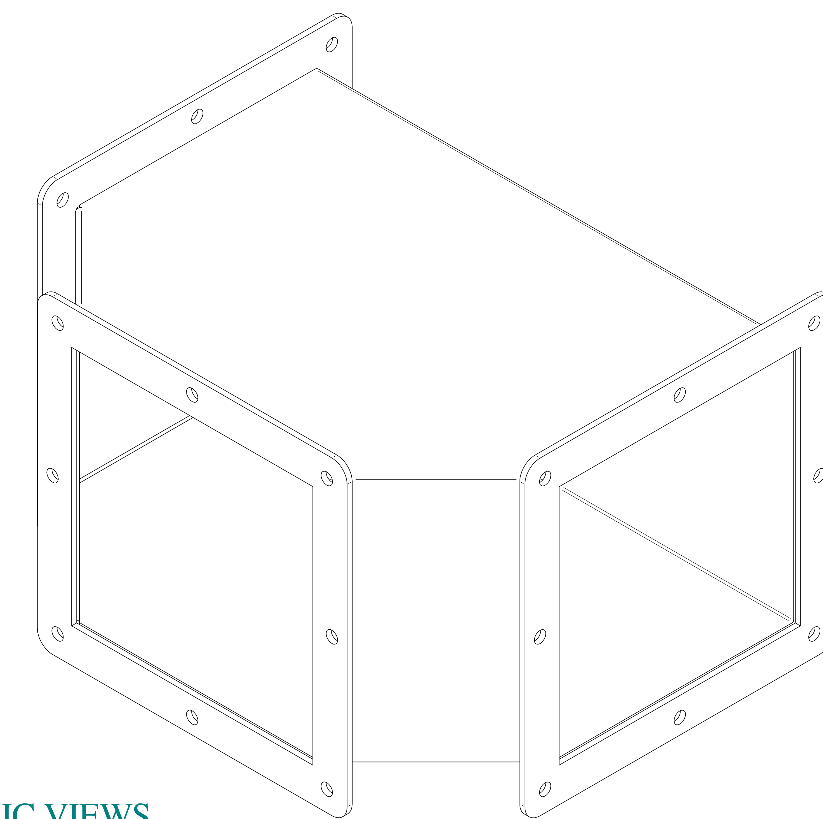
ISOMETRIC VIEWS
