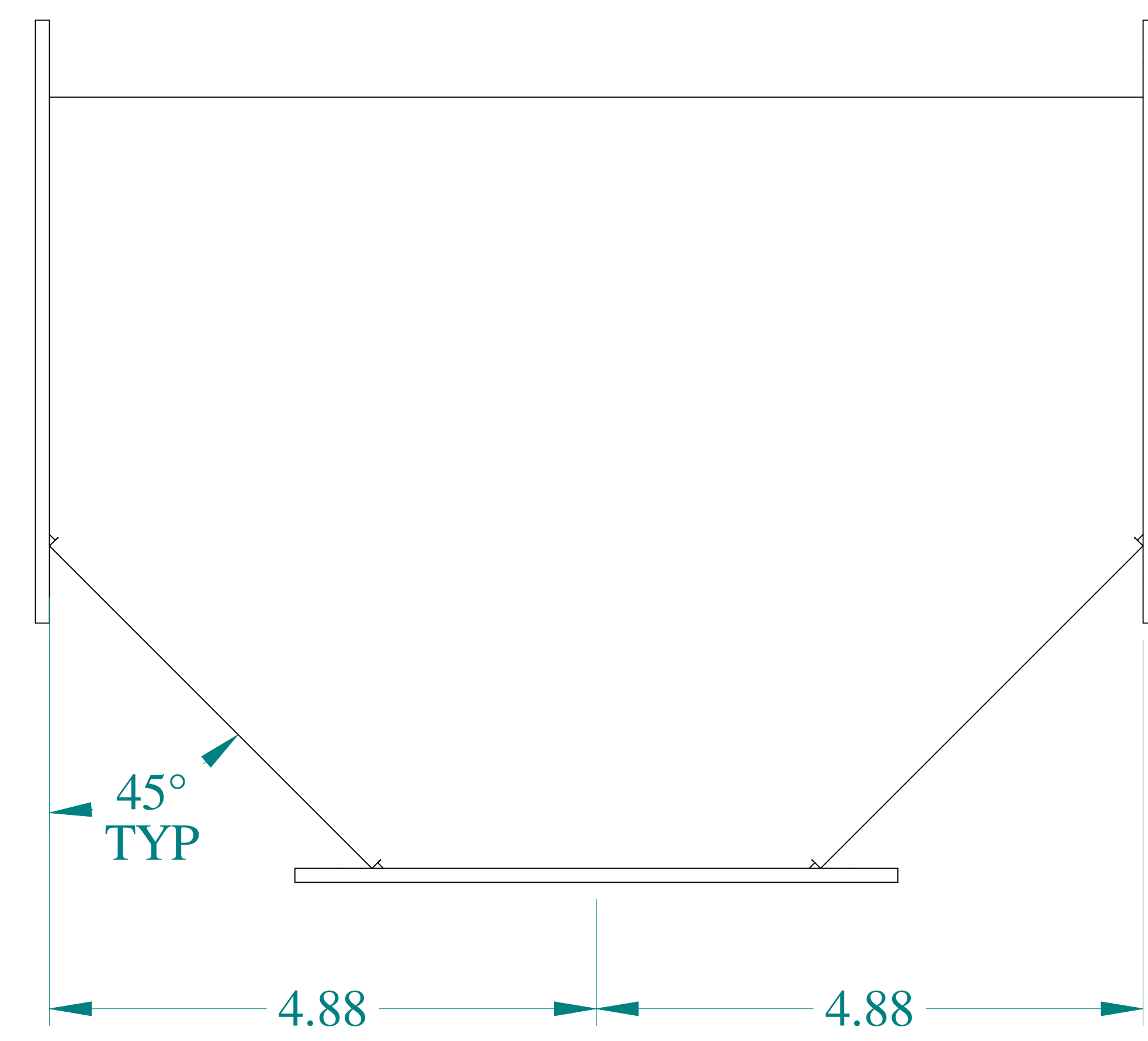
TOP VIEW
