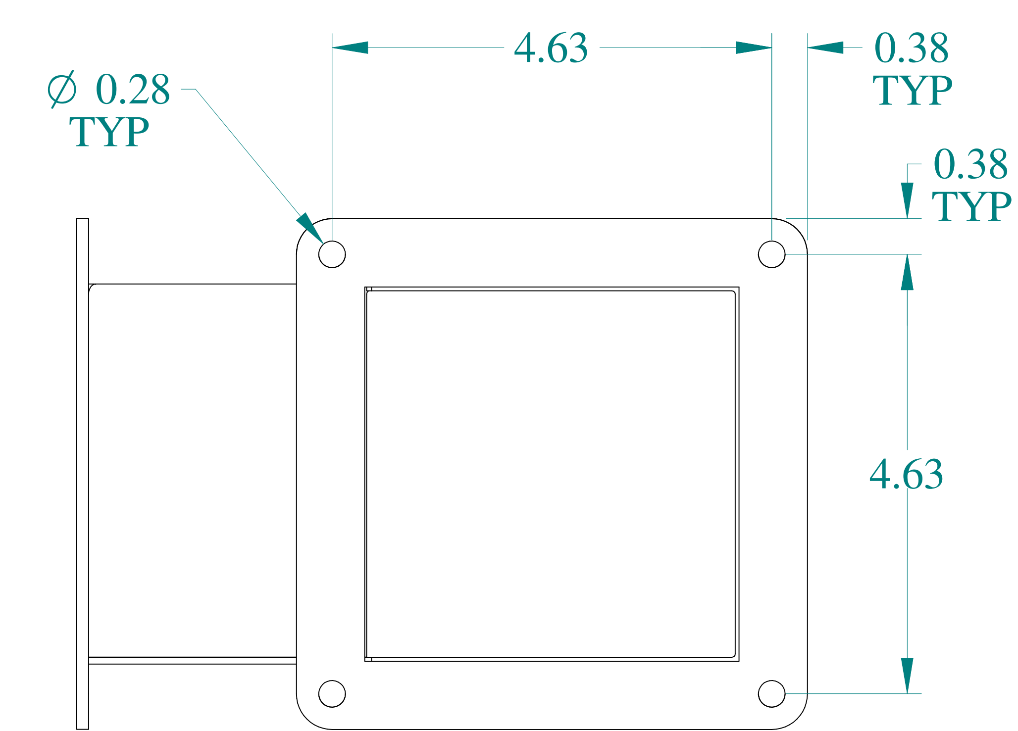
SIDE VIEW
