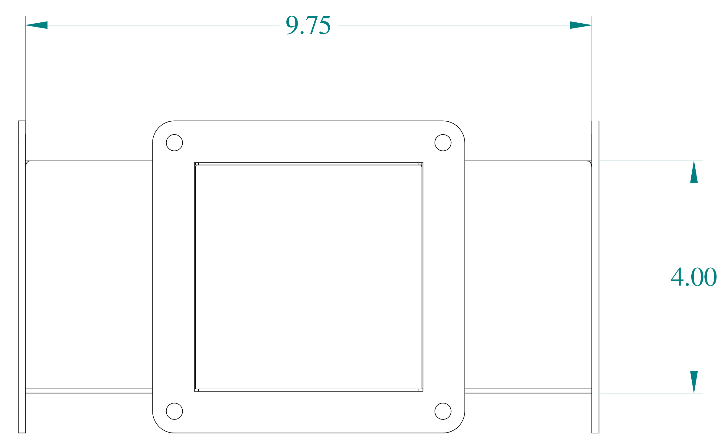
FRONT VIEW
