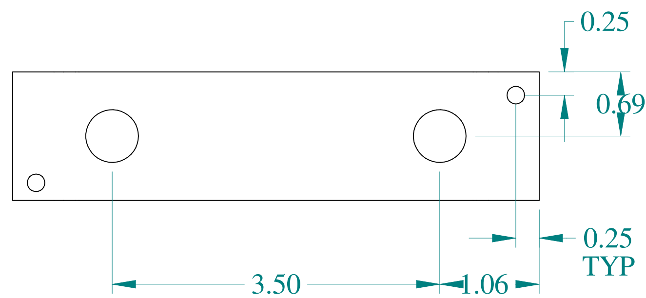
BOTTOM VIEW
