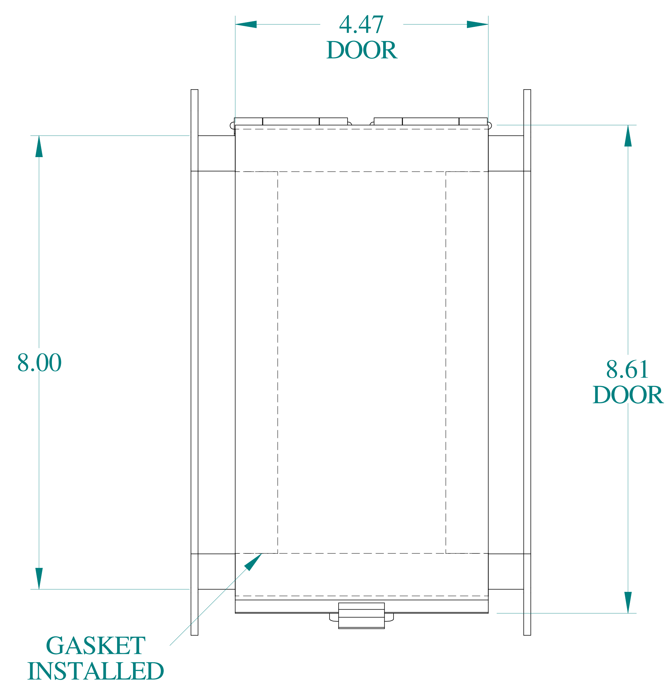
TOP VIEW
