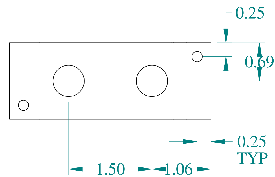
BOTTOM VIEW
