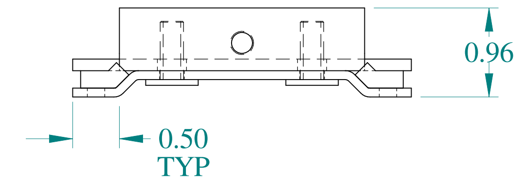
BACK VIEW
