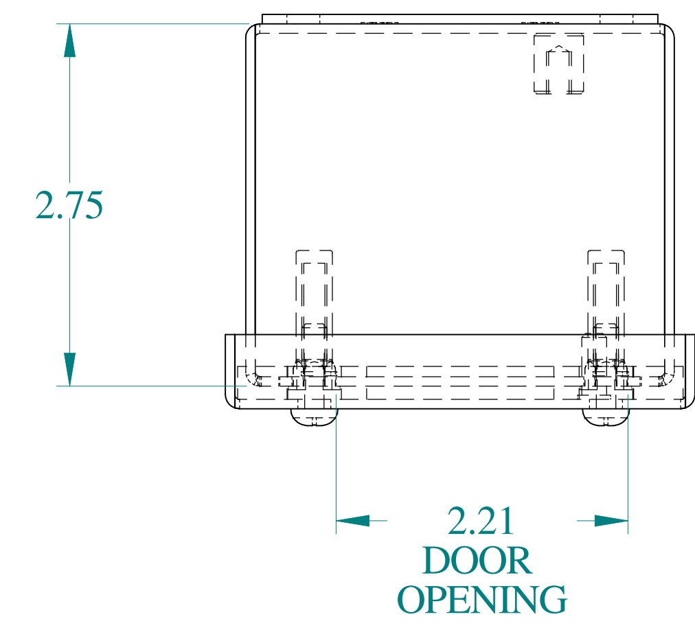
TOP VIEW
