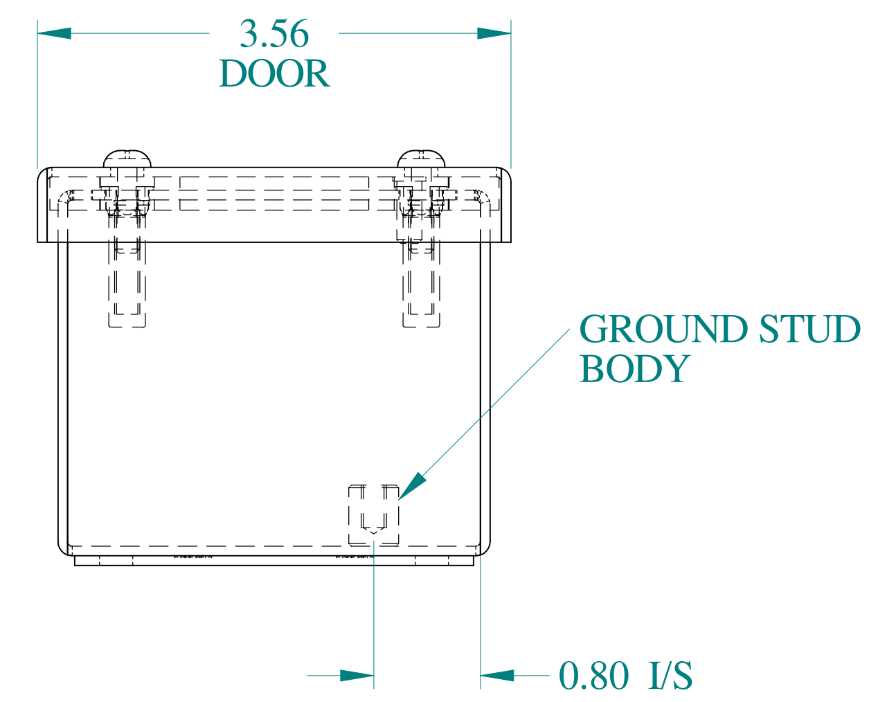
BOTTOM VIEW
