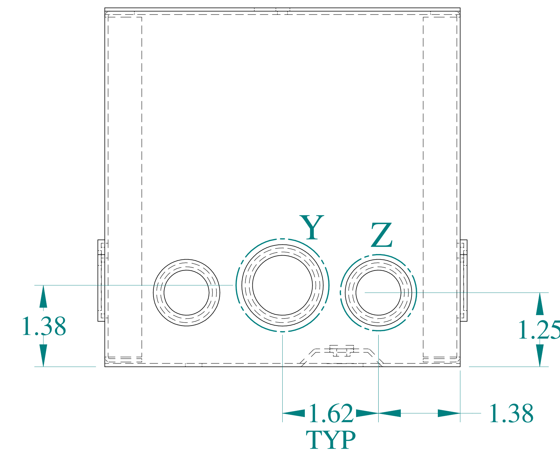
SIDE VIEW
