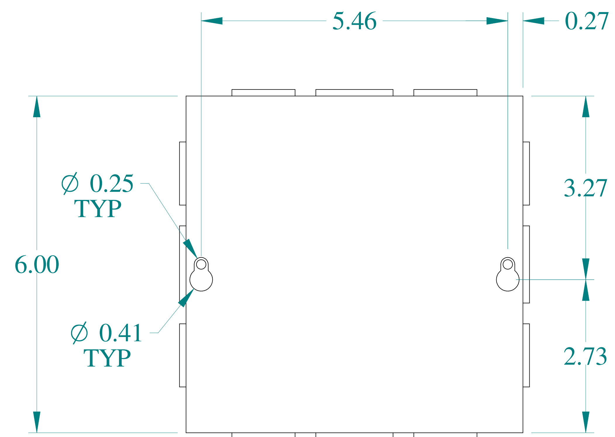
TOP VIEW
