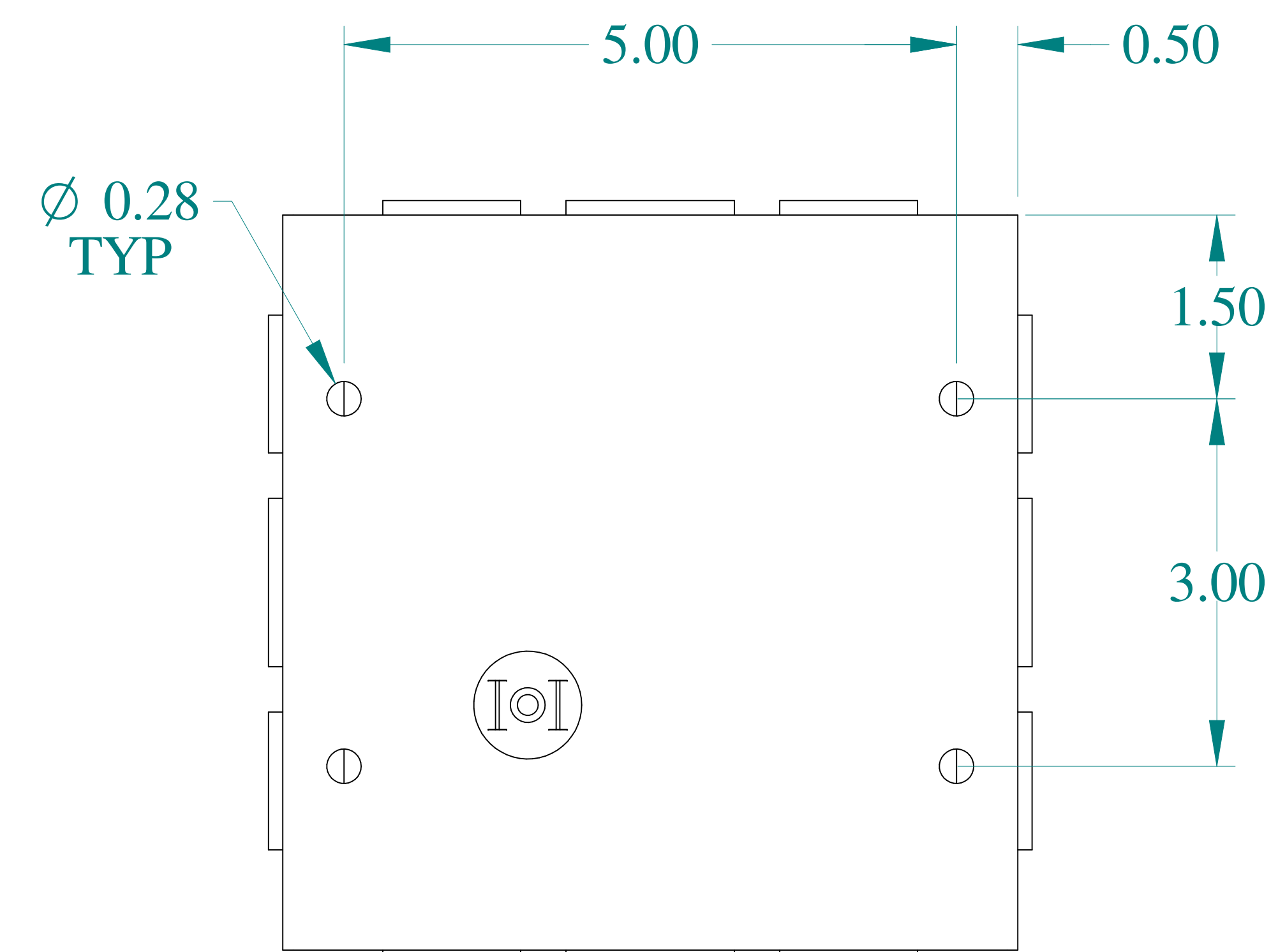
BOTTOM VIEW
