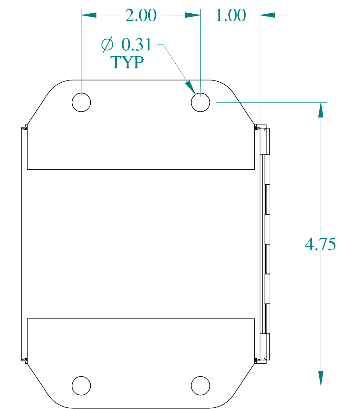
BACK VIEW
