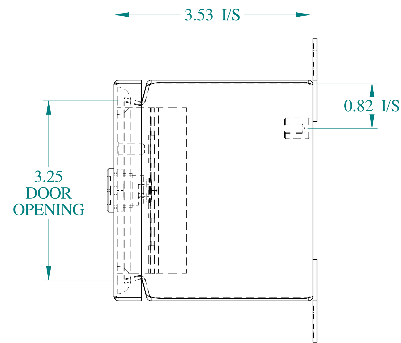
SIDE VIEW
