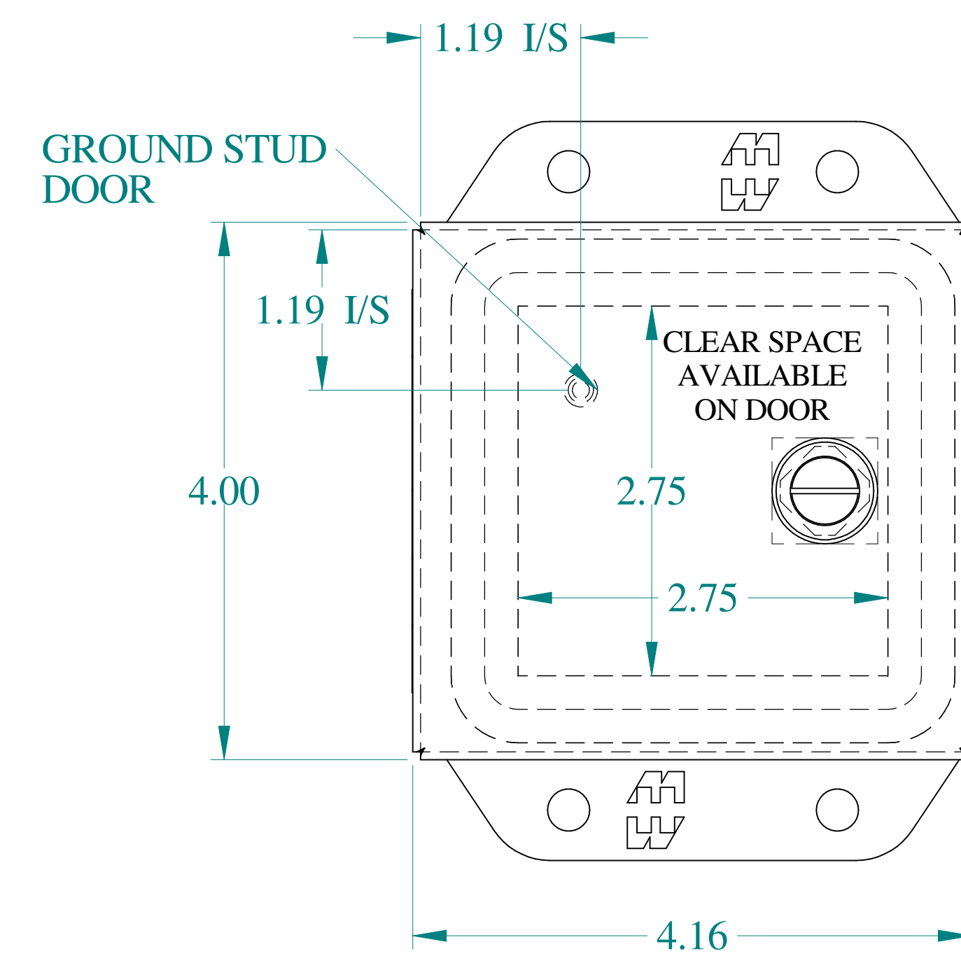
FRONT VIEW
