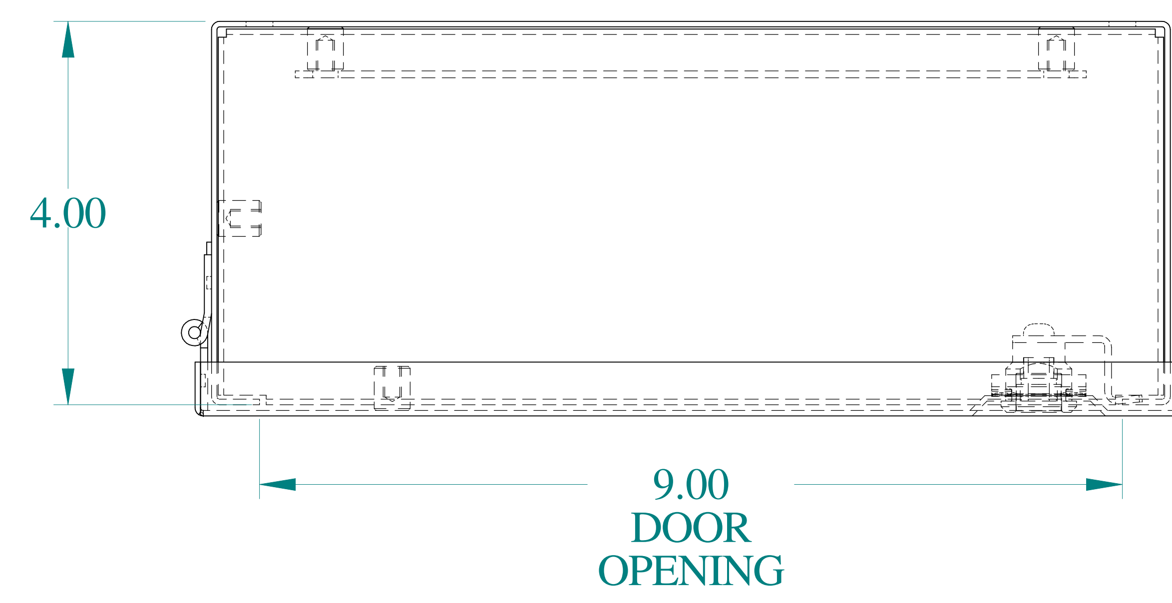
TOP VIEW
