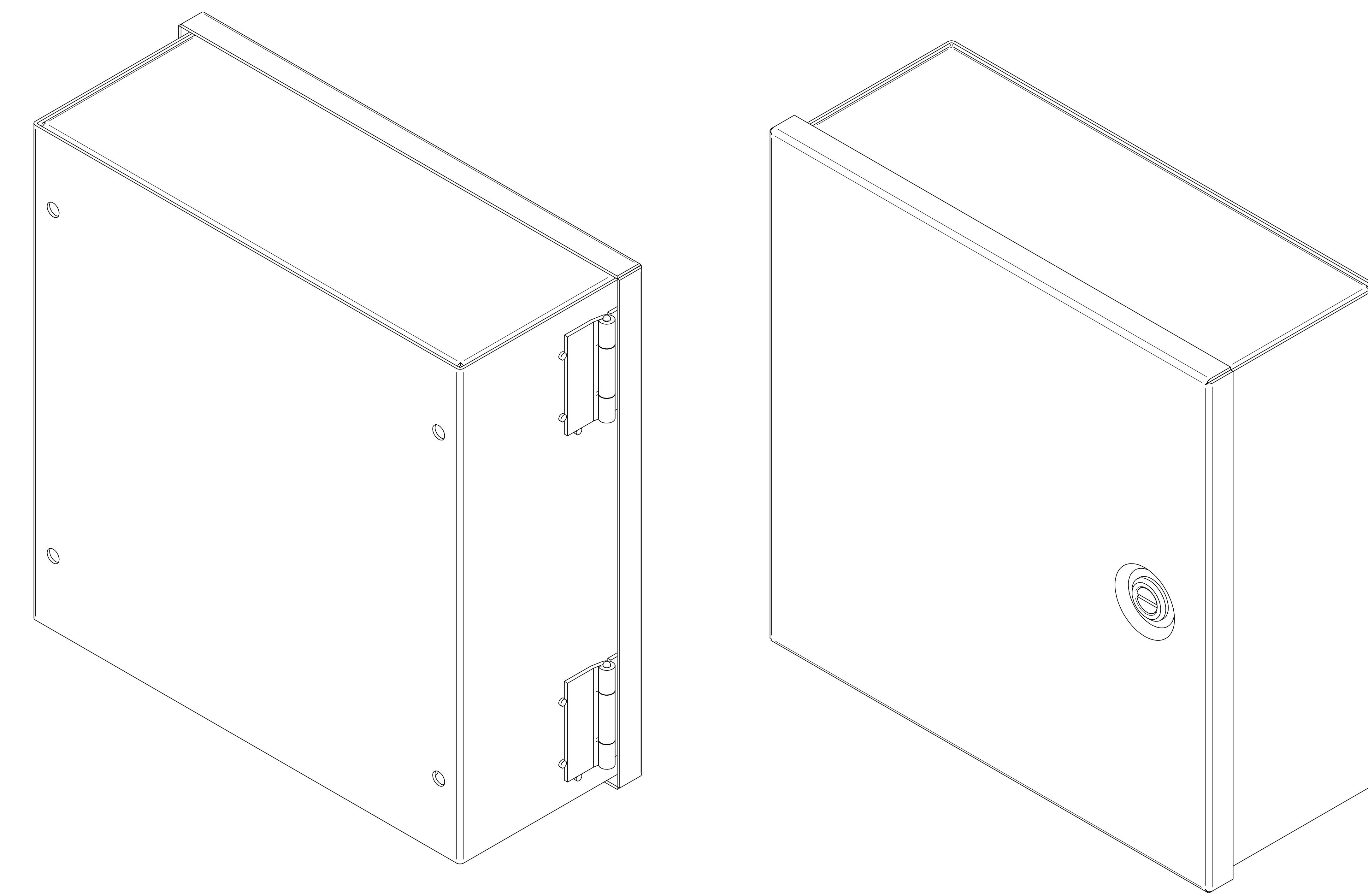
ISOMETRIC VIEWS
