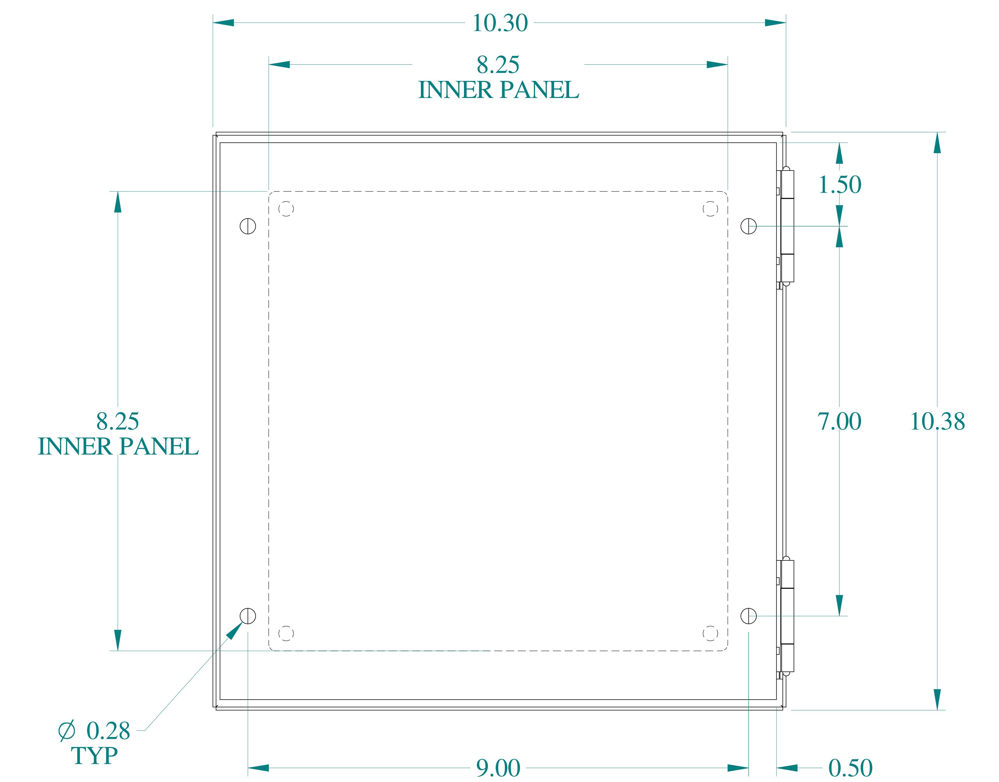
BACK VIEW
