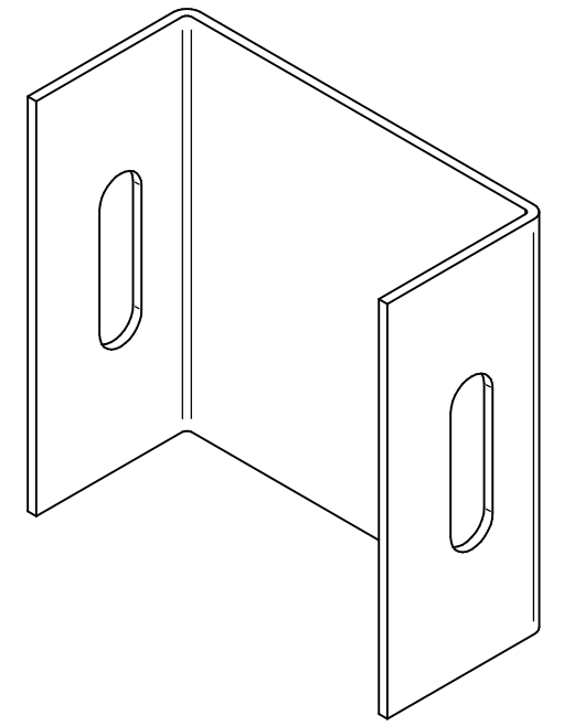
ISOMETRIC VIEWS
