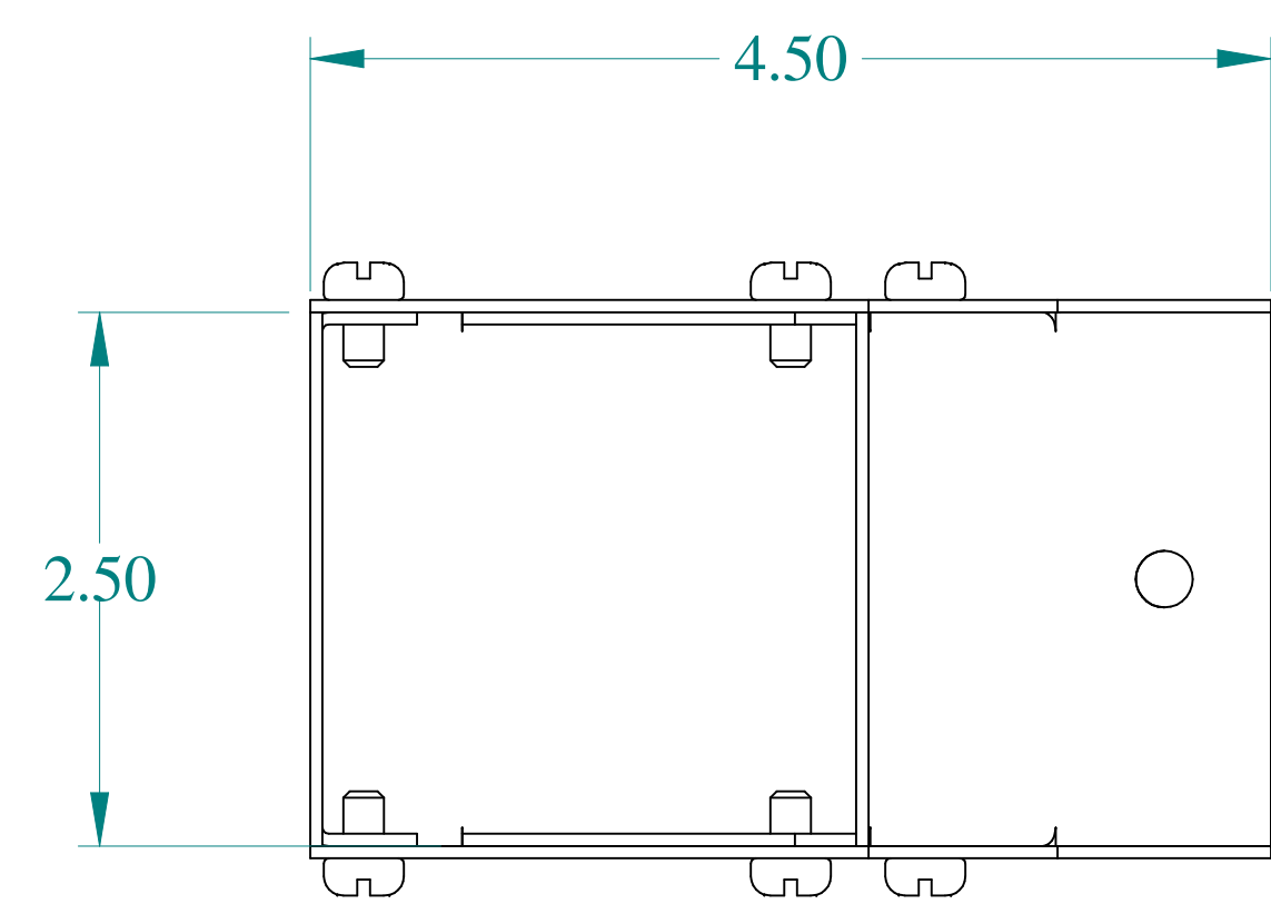
FRONT VIEW
