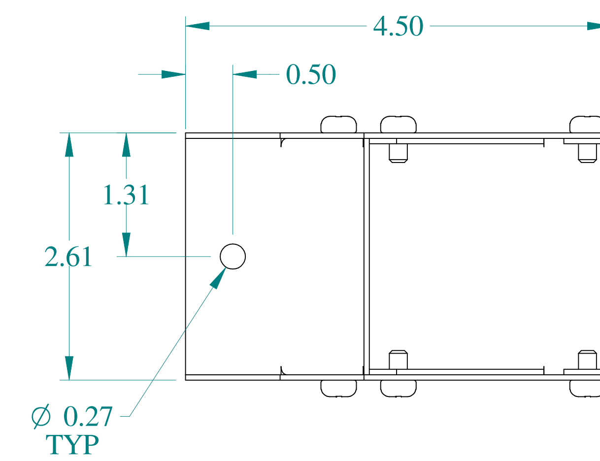
SIDE VIEW
