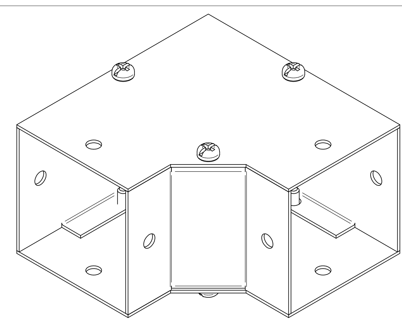
ISOMETRIC VIEWS
