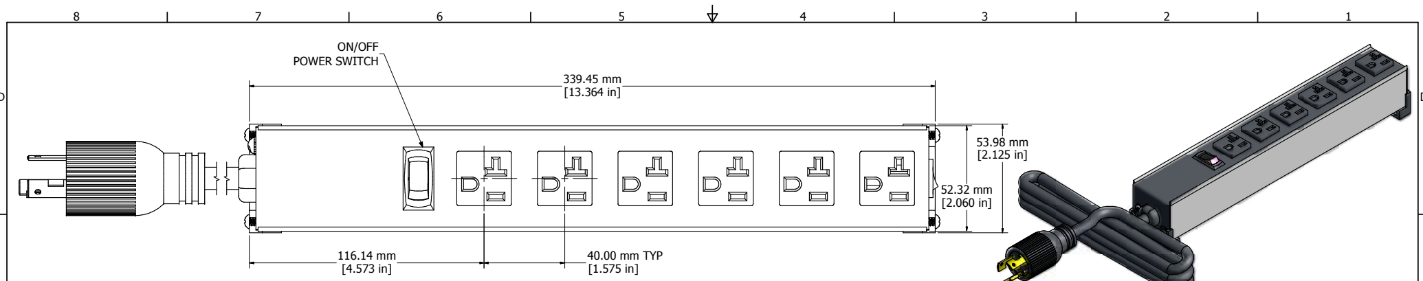
ASSEMBLY - VIEW FROM TOP
