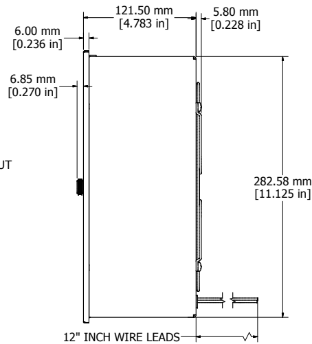
ASSEMBLY - VIEW FROM SIDE
