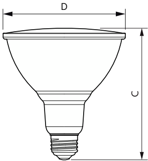
10PAR30S/LED/840/F40/DIM/ULW/120V 6/1FB
