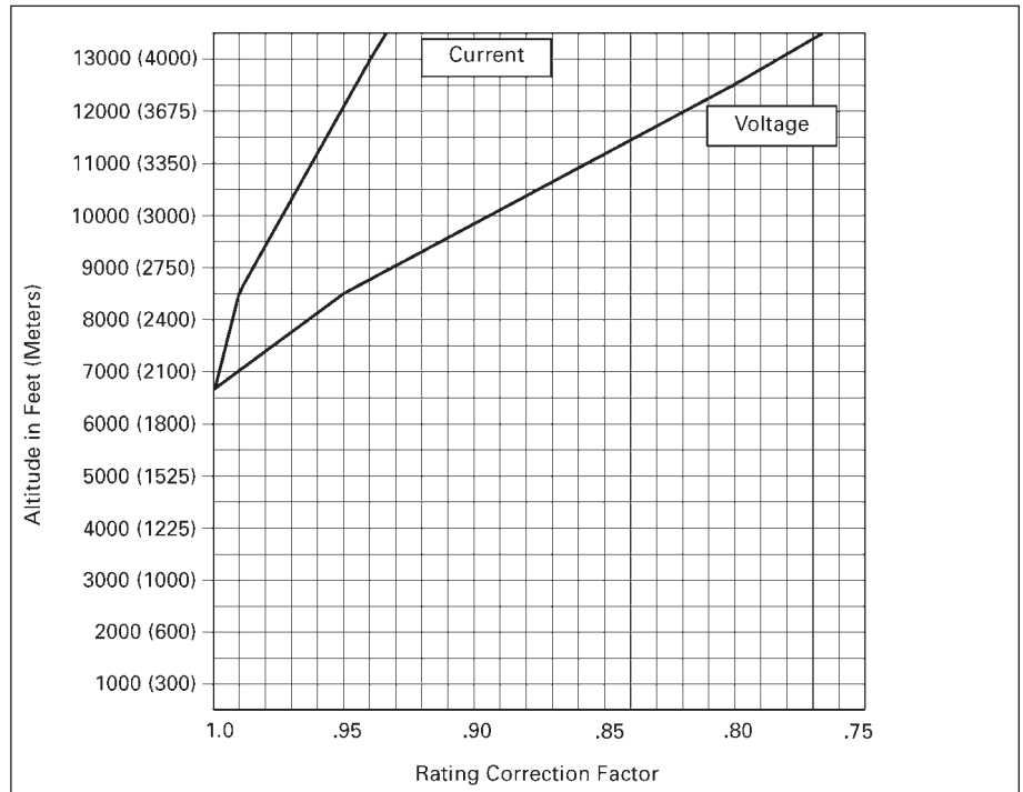
Figure 1 – Altitude adjustment
